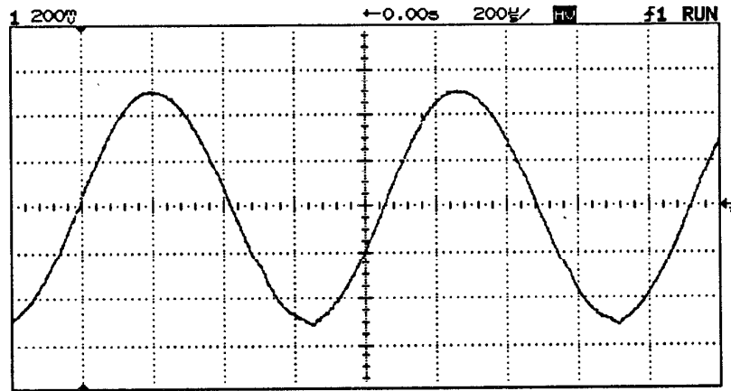
Delayed sweep isolates an area of interest for an rms voltage measurement
